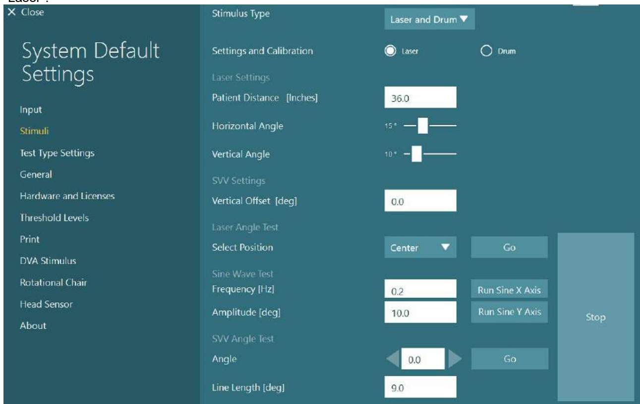
Figure 2.6-35: Laser stimuli settings for the Auto-Traverse/Comprehensive chair
